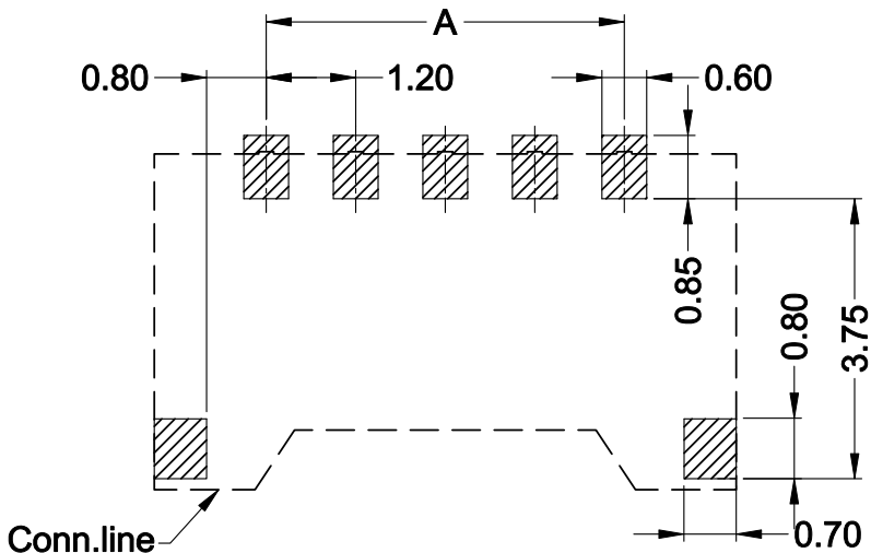
Recommended P.C.B Layout General Tolerance±0.05
